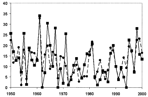
FIG. 5. The 1 Aug cross-validated hindcast (dashed line) of Sep hurricane days vs observations (solid line). Cross-validated (jackknifed) variance ( r^2 ) explained is 0.51.
